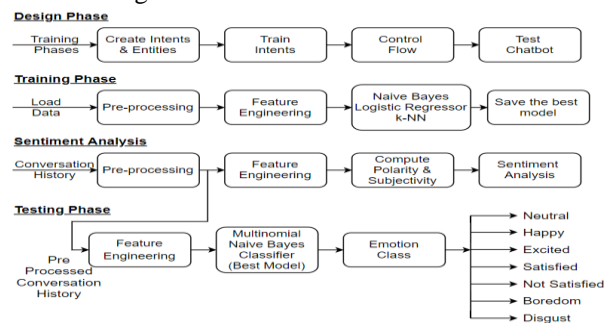
Figure 2. System Architecture
