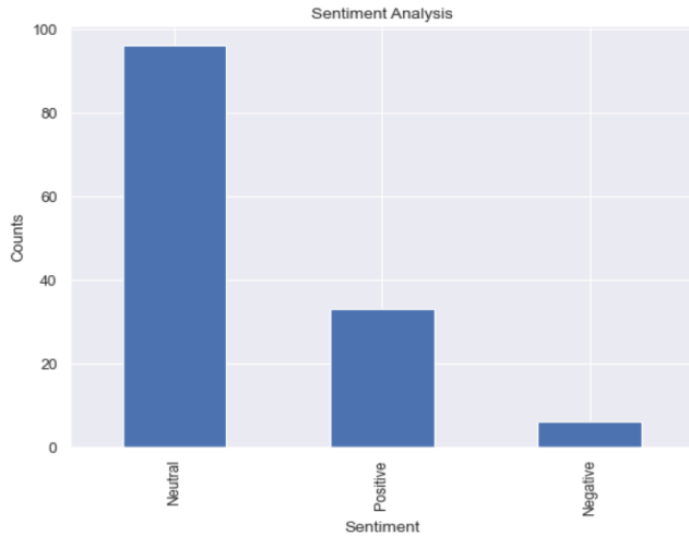
Figure 6. Sentiment Analysis
