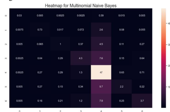
Figure 9. Confusion Matrix of the Proposed System for Multinomial Naive Bayes Classifier
